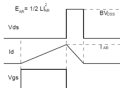
Fig.3-2 Avalanche waveform
