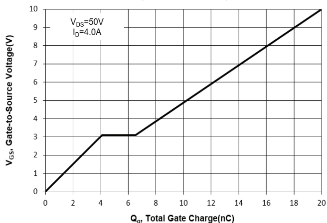
Fig. 11 Gate Charge
