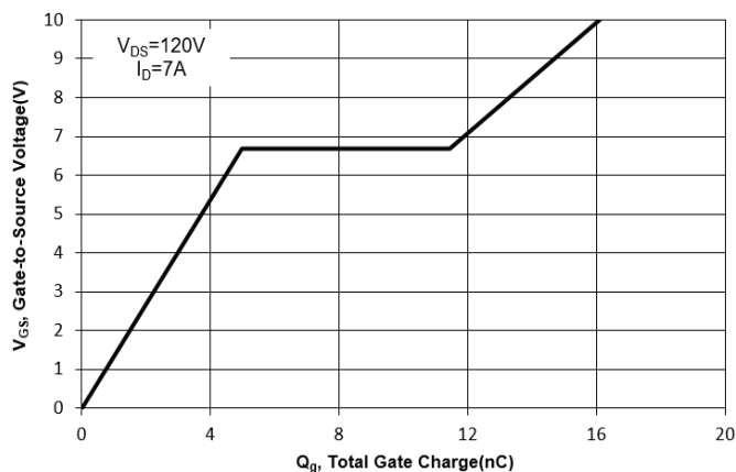
Fig. 11 Gate Charge
