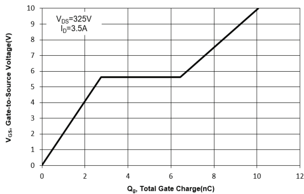
Fig. 11 Gate Charge
