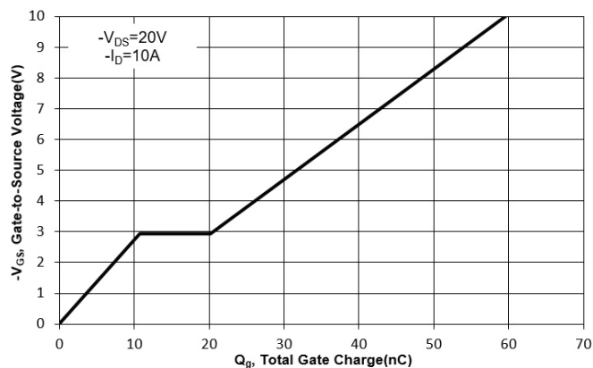
Fig. 11 Gate Charge
