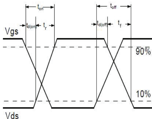
Fig.1-2 Switching Waveform
