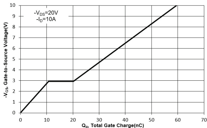
Fig. 11 Gate Charge
