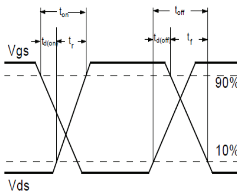
Fig.1-2 Switching Waveform
