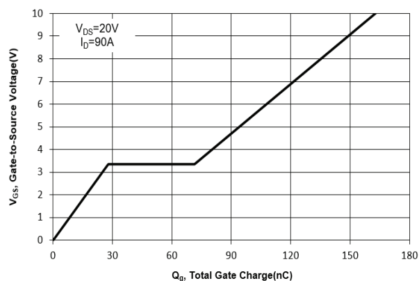
Fig. 11 Gate Charge
