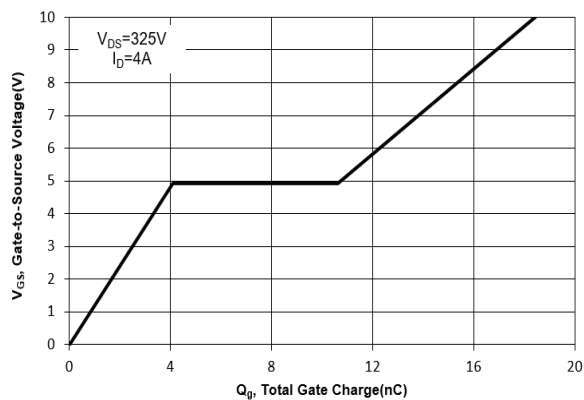
Fig. 11 Gate Charge
