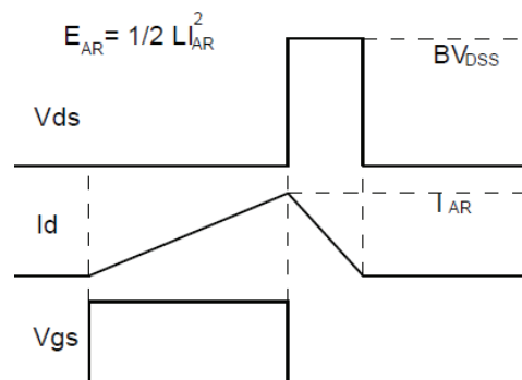
Fig.3-2 Avalanche waveform
