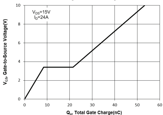
Fig. 11 Gate Charge
