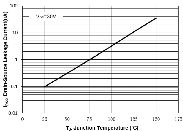
Fig. 8 Drain-Source Leakage Current vs. T_j
