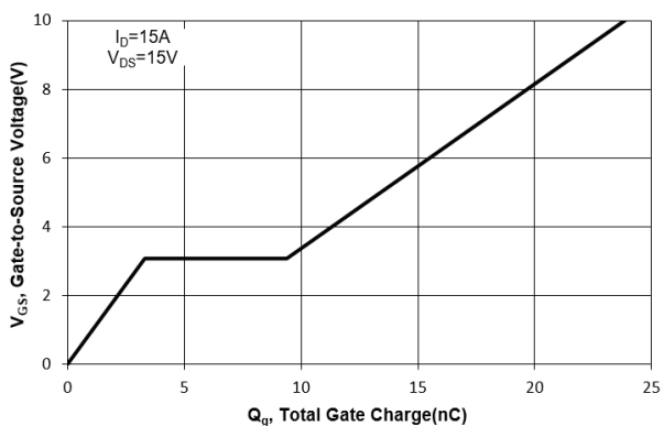
Fig. 11 Gate Charge
