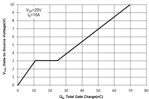
Fig. 11 Gate Charge
