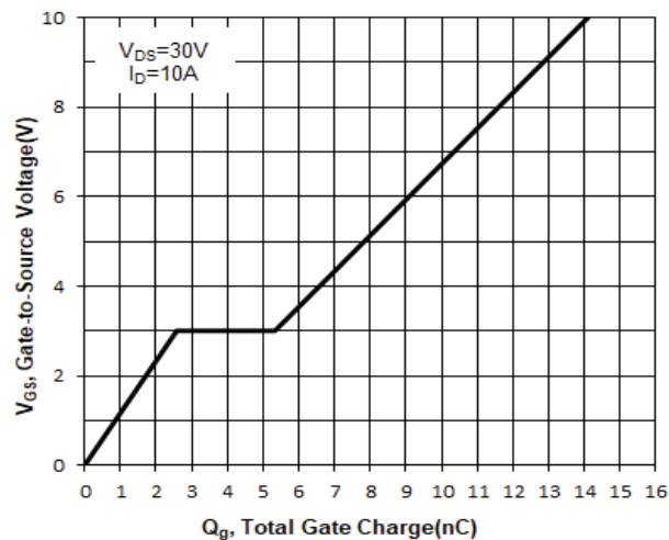
Fig 10. Gate Charge
