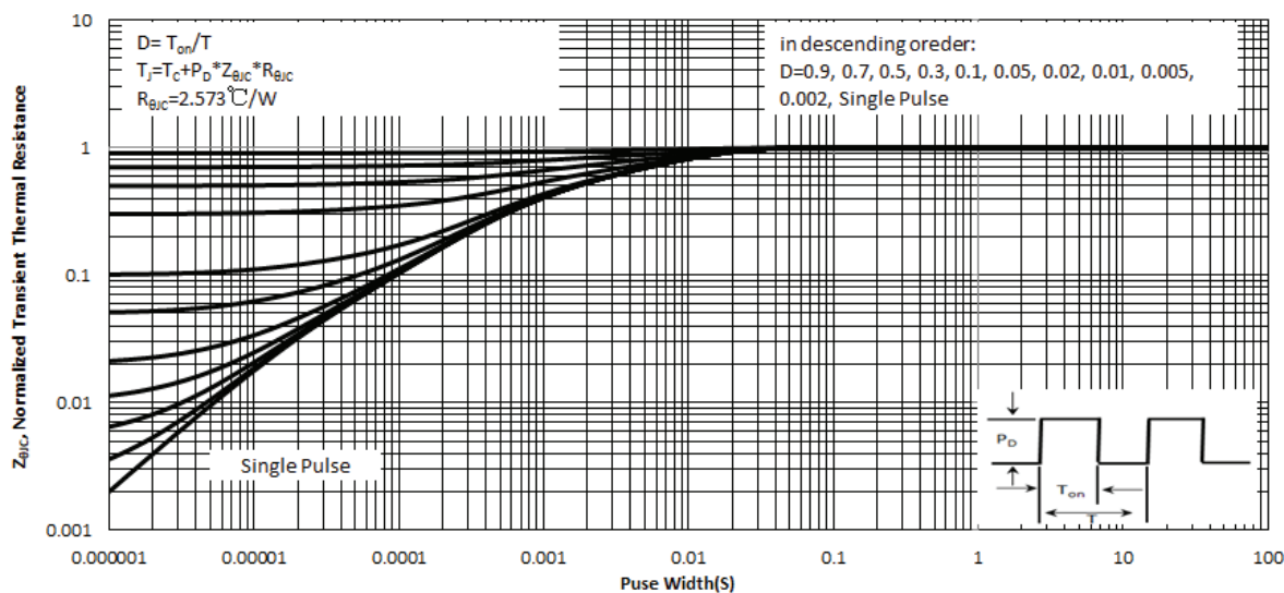
Fig.12 Normalized Maximum Transient Thermal Impedance( Z_{\theta JC} )
