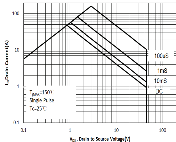
Fig.6 Safe Operation Area
