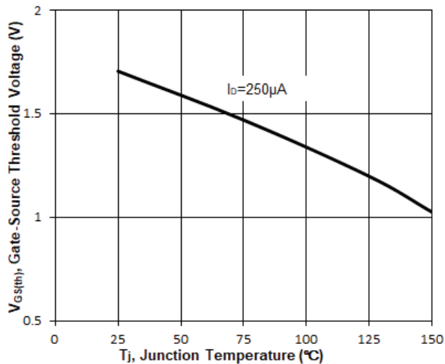
Fig.7 Gate Threshold Voltage vs. T_j
