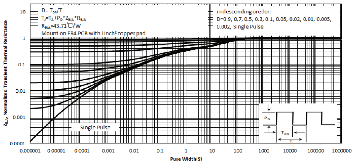
Fig.11 Normalized Maximum Transient Thermal Impedance( Z_{\theta JA} )
