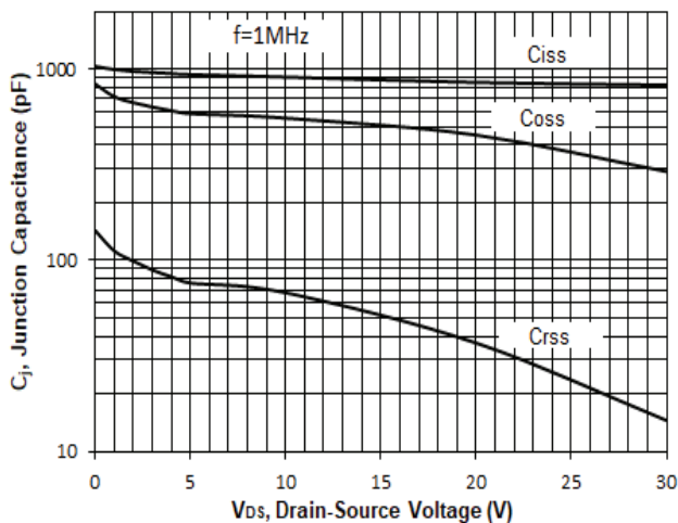
Fig 9. Capacitance Characteristic
