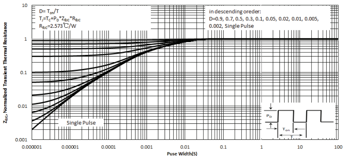
Fig.12 Normalized Maximum Transient Thermal Impedance( Z_{\theta JC} )
