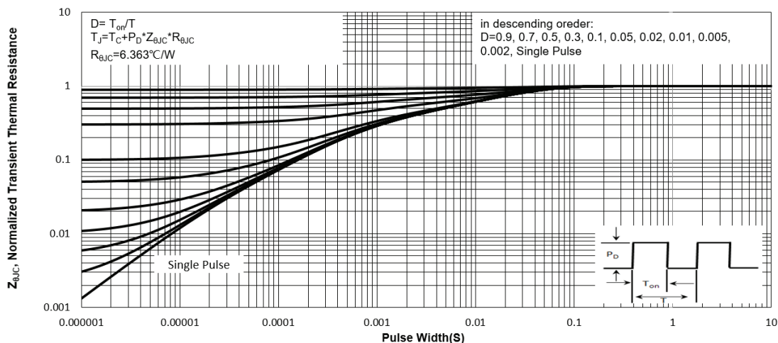
Fig. 13 Normalized Maximum Transient Thermal Impedance( z_{\theta JC} )
