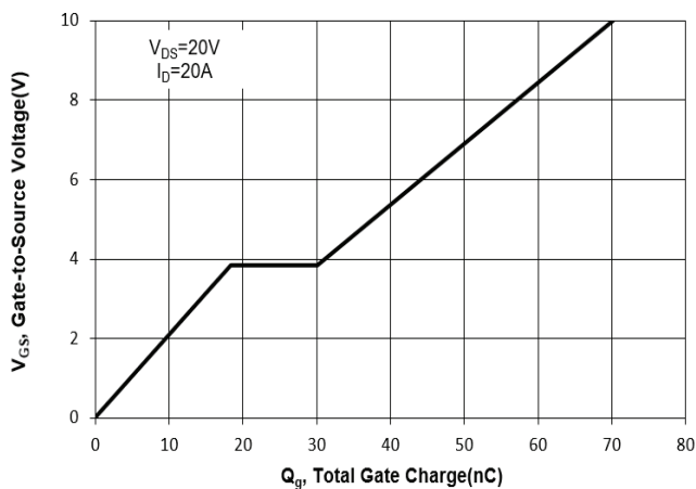
Fig. 11 Gate Charge
