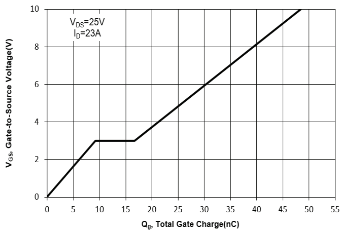
Fig. 11 Gate Charge
