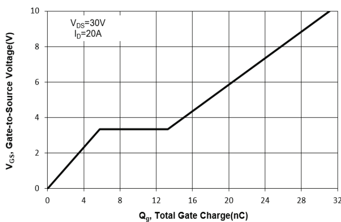
Fig. 11 Gate Charge
