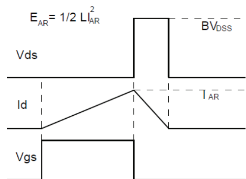
Fig.3-2 Avalanche waveform
