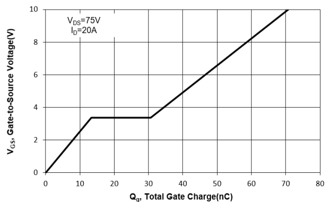
Fig. 11 Gate Charge
