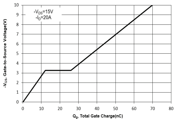
Fig. 11 Gate Charge
