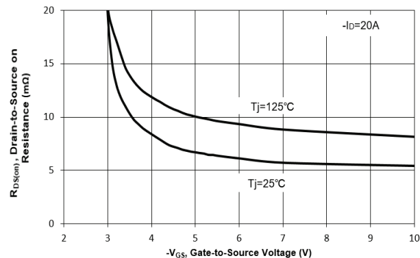
Fig. 4 on-Resistance vs. Gate Voltage
