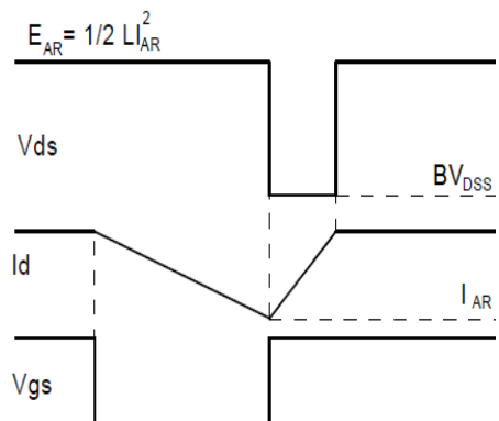
Fig.3-2 Avalanche waveform
