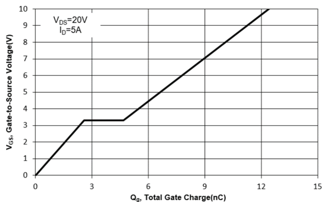
Fig. 11 Gate Charge
