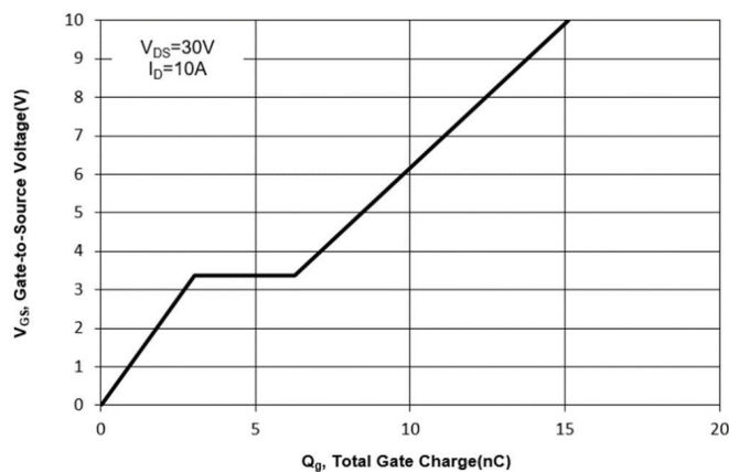
Fig. 11 Gate Charge
