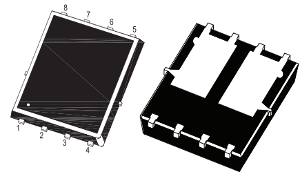
Q1: 1.Gate 2. Source 7.Drain 8.Drain Q2: 3.Source 4.Gate 5.Drain 6.Drain DFN5060 Plastic Package
