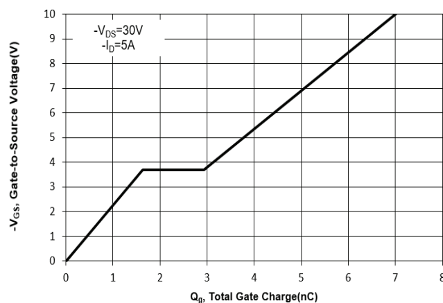
Fig. 11 Gate Charge
