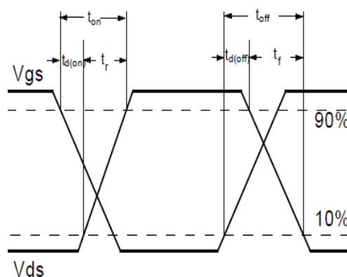
Fig.1-2 Switching Waveform
