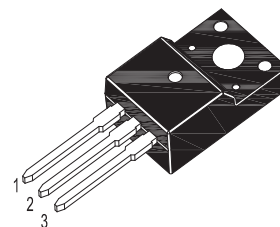
TO-220F Plastic Package 1.Gate 2.Drain 3.Source
