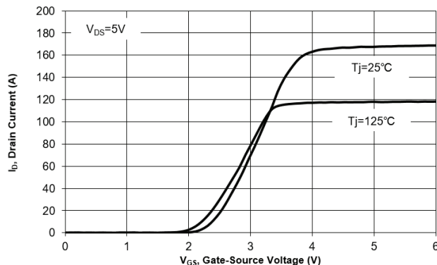
Fig. 2 Typical Transfer Characteristics
