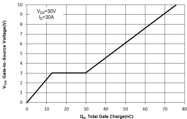
Fig. 11 Gate Charge
