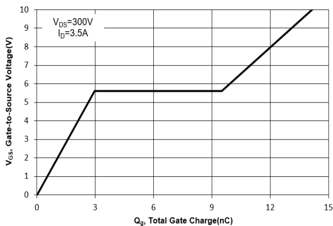
Fig. 11 Gate Charge
