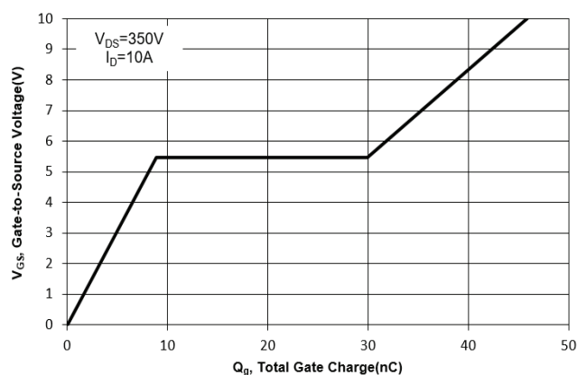
Fig. 11 Gate Charge
