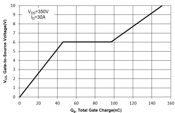
Fig. 11 Gate Charge
