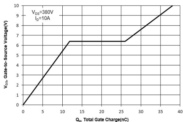
Fig. 11 Gate Charge
