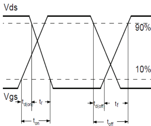
Fig.1-2 Switching Waveform
