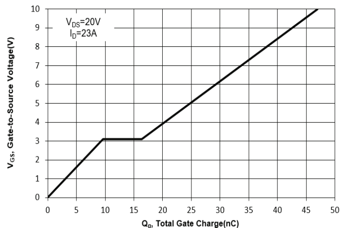
Fig. 11 Gate Charge
