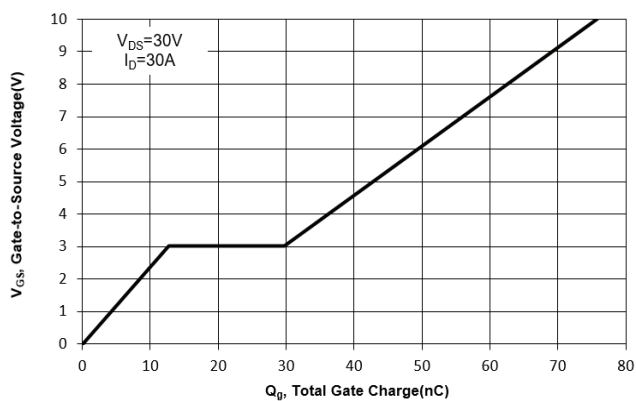
Fig. 11 Gate Charge
