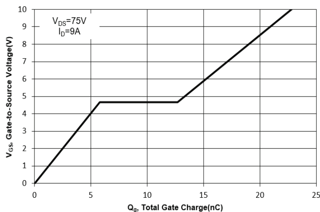
Fig. 11 Gate Charge
