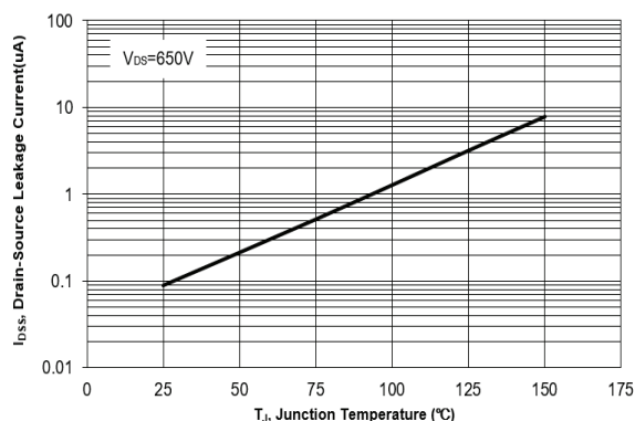
Fig. 8 Drain-Source Leakage Current vs. T_J
