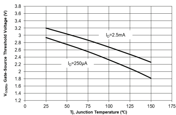
Fig. 10 Gate Threshold Variation vs. T_J
