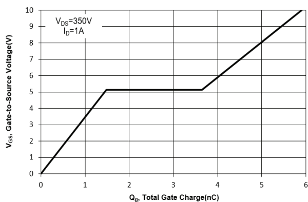
Fig. 11 Gate Charge
