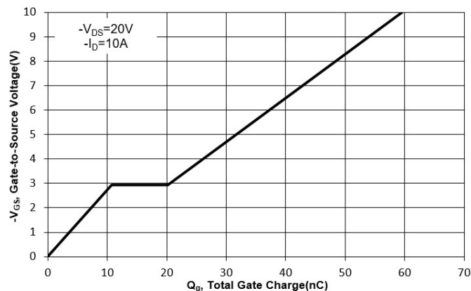
Fig. 11 Gate Charge
