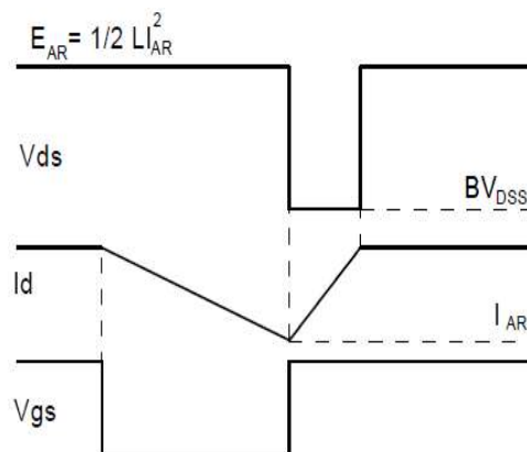
Fig.3-2 Avalanche waveform
