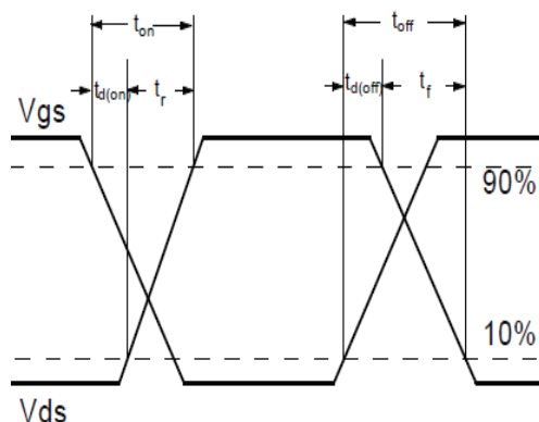
Fig.1-2 Switching Waveform
