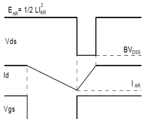
Fig.3-2 Avalanche waveform
