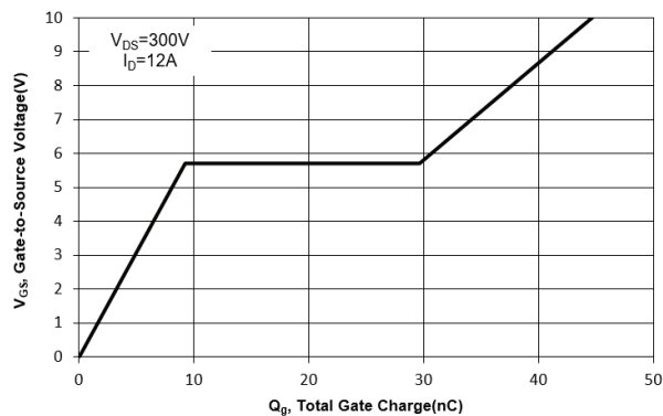
Fig. 11 Gate Charge
