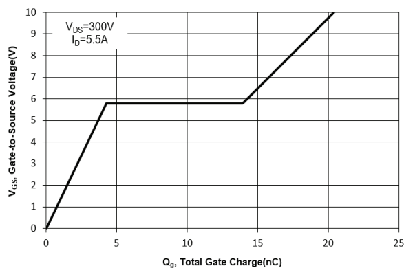
Fig. 11 Gate Charge
