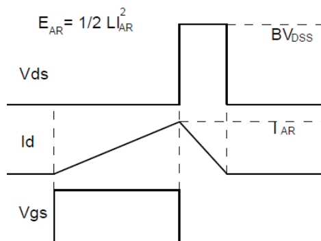
Fig.3-2 Avalanche waveform
