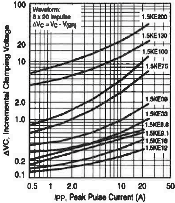
Fig. 7 – Incremental Clamping Voltage Curve (Unidirectional)
