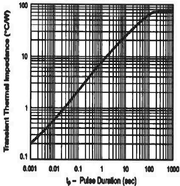
Fig. 13 - Typical Transient Thermal Impedance
