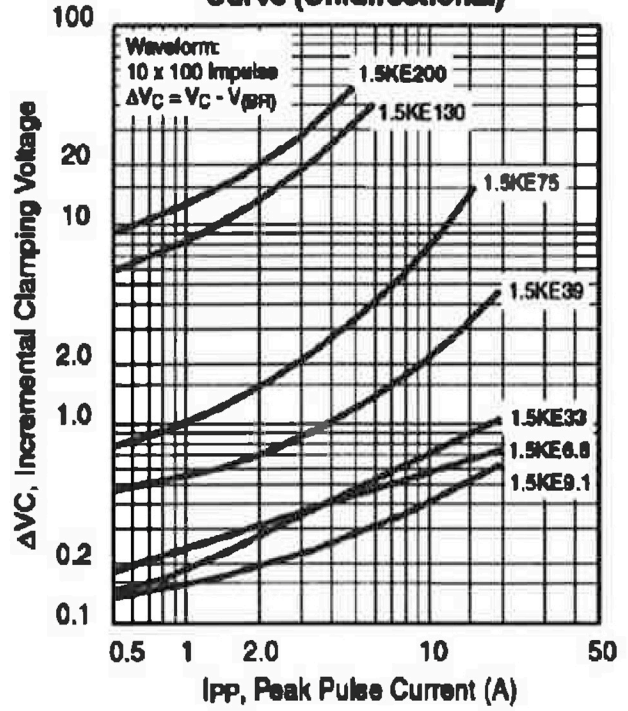
Fig. 8 – Incremental Clamping Voltage Curve (Unidirectional)
