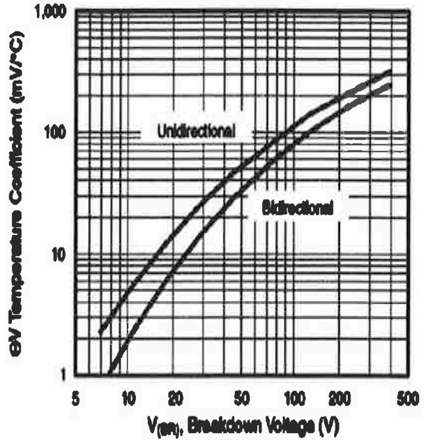
Fig. 12 - Breakdown Voltage Temperature Coefficient Curve
