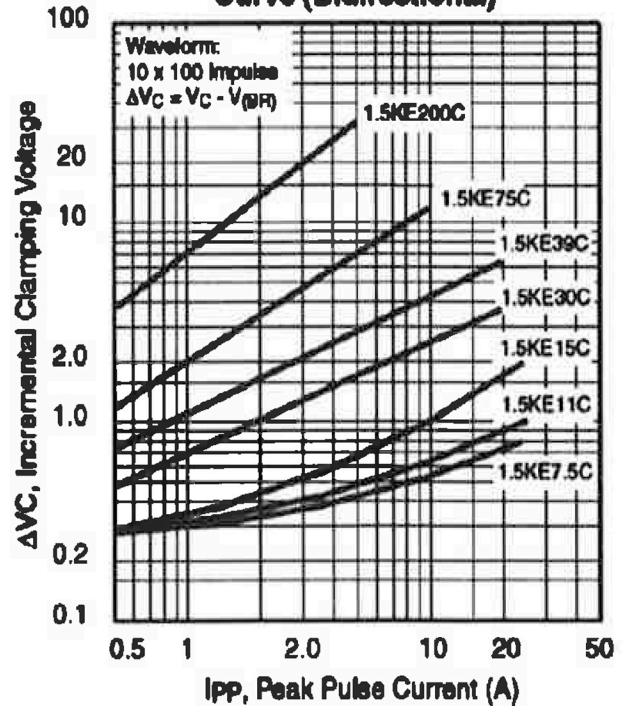
Fig. 10 – Incremental Clamping Voltage Curve (Bidirectional)
