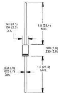
DO-204AC (DO-15)
