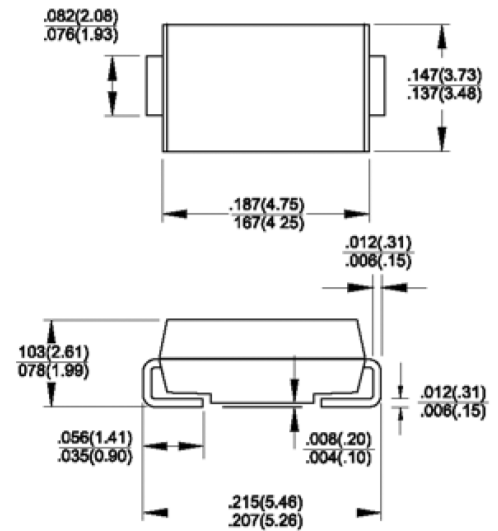
DO-214AA (SMB)
