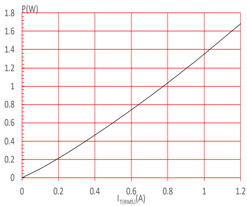
FIG.1: Maximum power dissipation versus RMS on-state current
